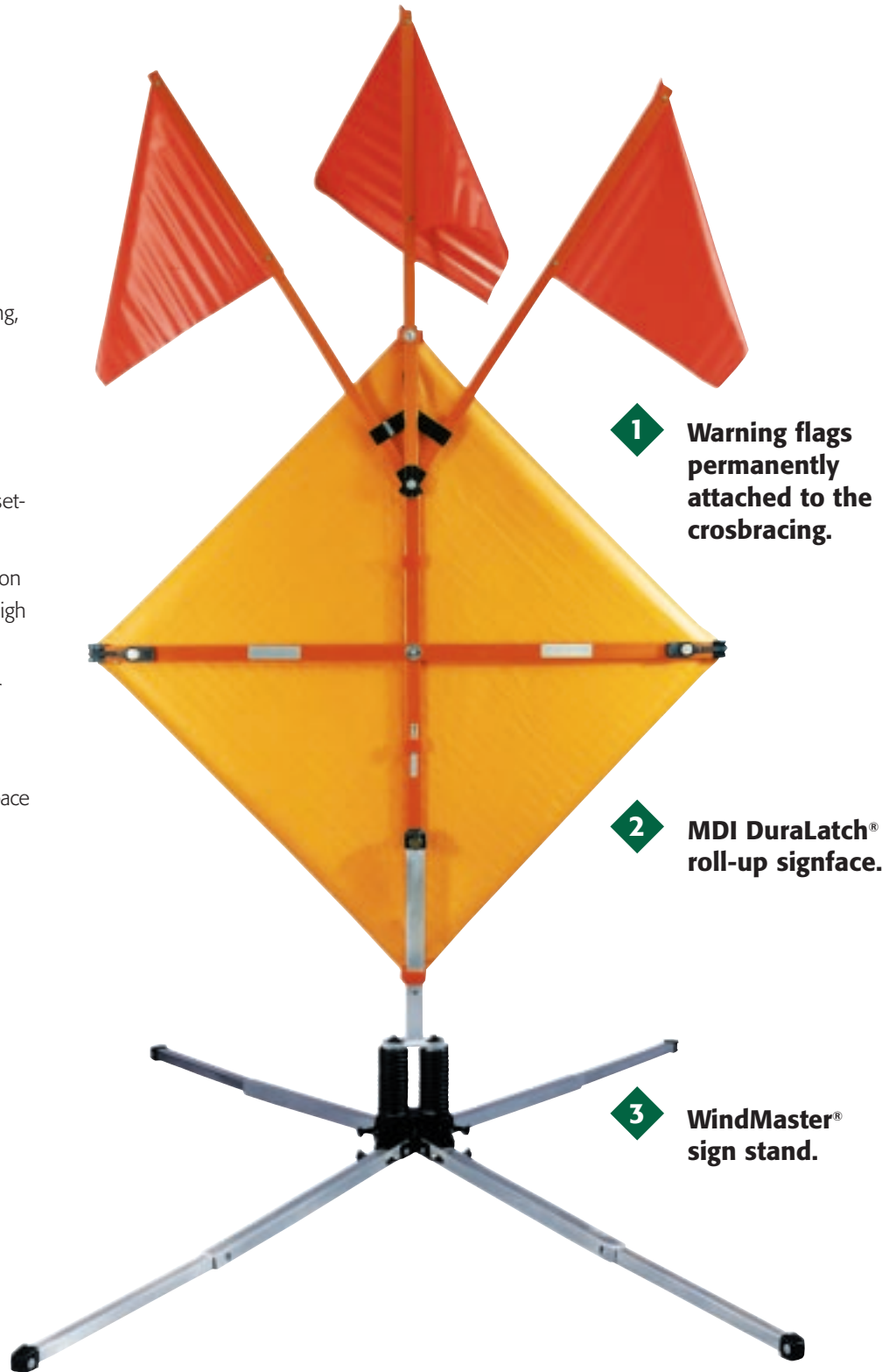
The patented design allows the worker to remain upright, increasing traffic visibility.
